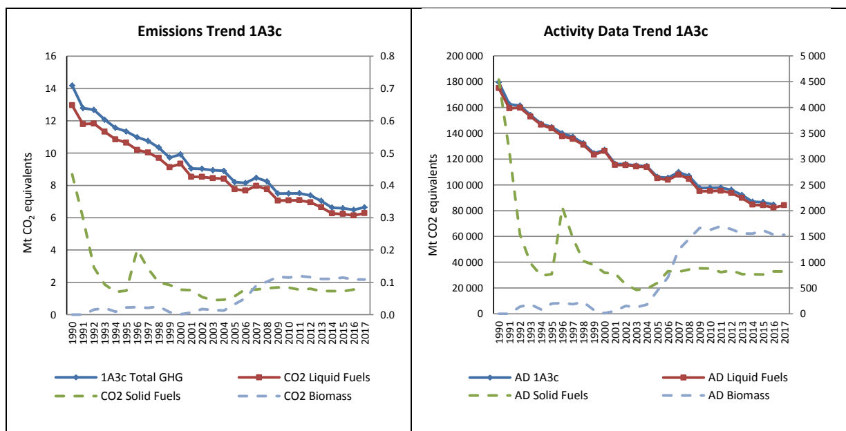
Figure 3.132 1A3c Railways: CO 2 Emission Trend and Activity Data
