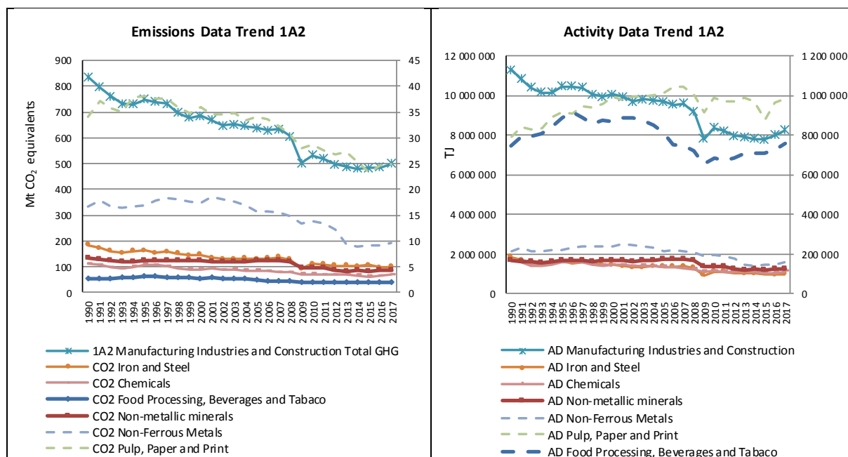
Figure 3.30: 1A2 Manufacturing Industries and Construction: Total and CO 2 emission trends
