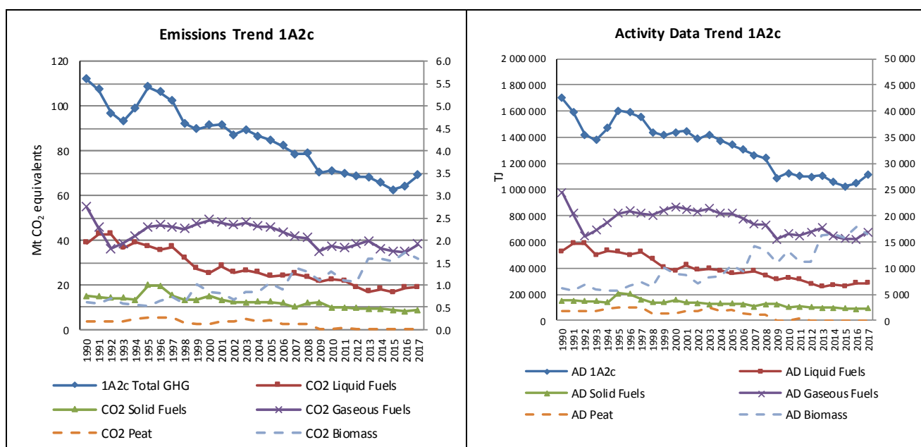
Figure 3.51: 1A2c Chemicals: Total and CO 2 emission and activity trends
