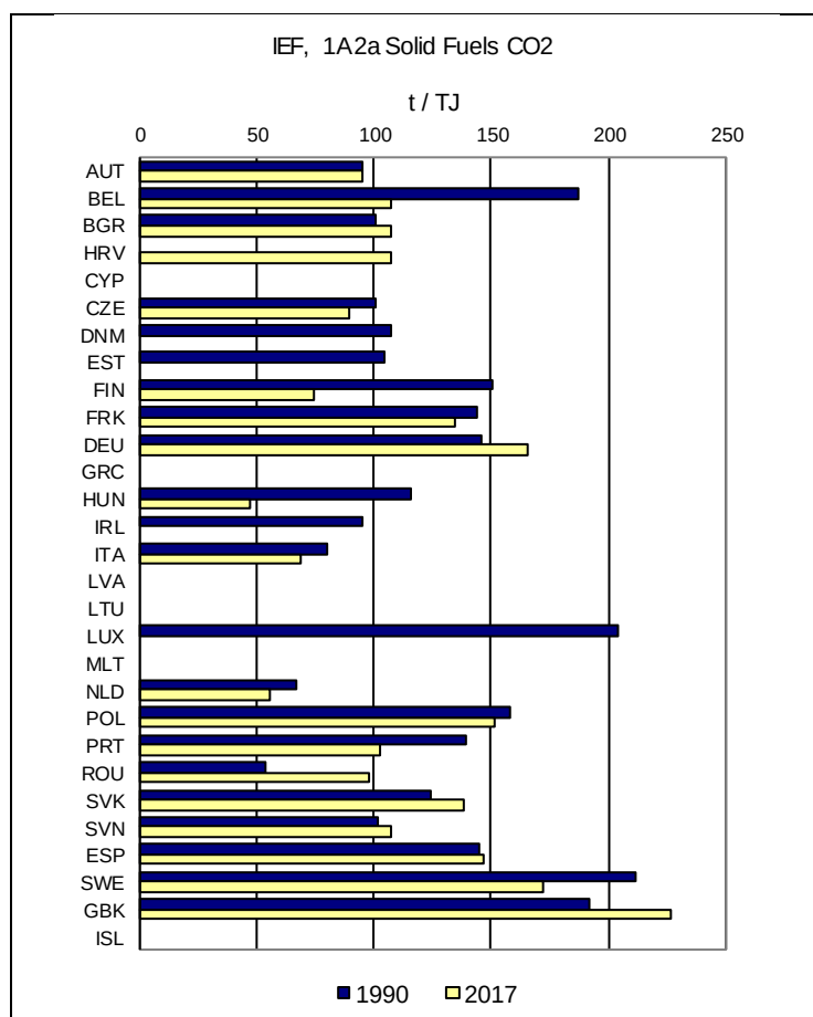
Figure 3.37: 1A2a Iron and Steel, Solid fuels: Implied Emission Factors for CO 2 by Member States and Iceland (in t/TJ)
