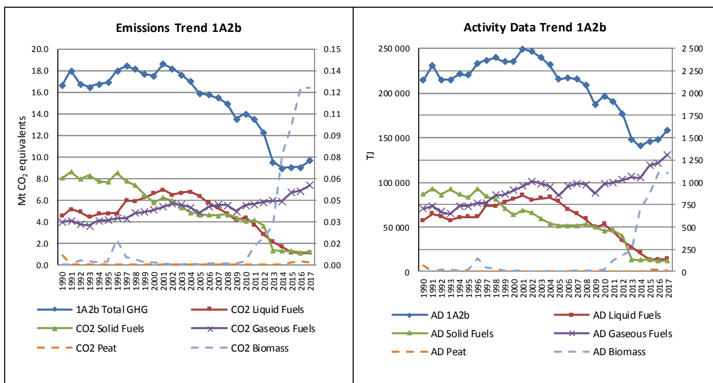
Figure 3.41: 1A2b Non-ferrous Metals: CO 2 emissions and activity data trends
